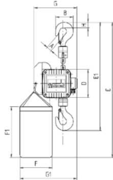
OVERALL DIMENSIONS - WEIGHTS
