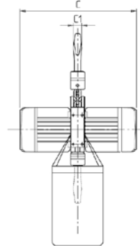
OVERALL DIMENSIONS - WEIGHTS
