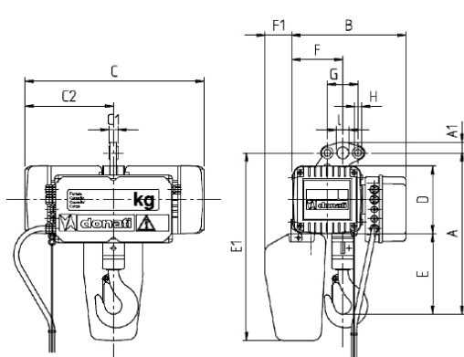
1 chain fall version
