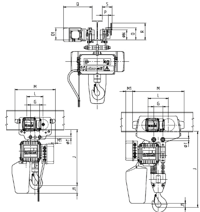
1 chain fall version
