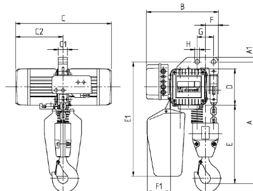
2 chain falls version
